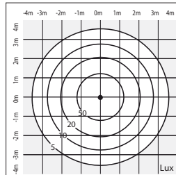
S7175 - 1x 35 MT G12 H=1 m
