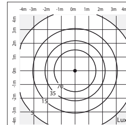
S7176 - 1x 70 MT G12 H=1 m
